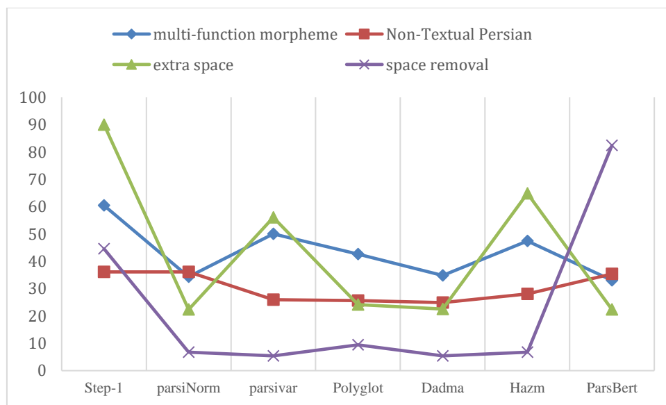
Figure 6: Comparison of tokenizer accuracy relative to phenomena
