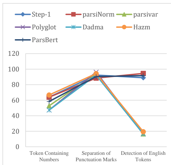
Figure 3 : Comparison of tokenizer Accuracy for non-textual Persian
